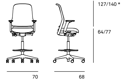
164/1 Counter chair
