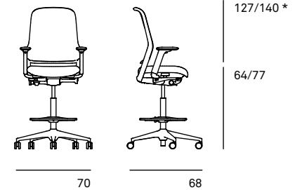
165/1 Counter chair
